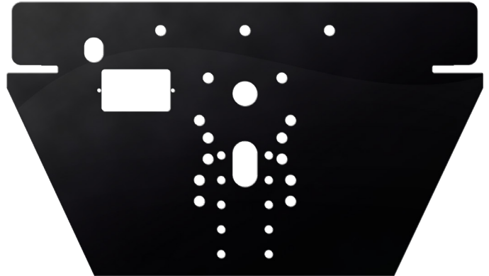
HTE336 19.50" x 33.88" overall 3/4" thick steel - For tandem axle MINIMUM ORDER QUANTITY: 1
