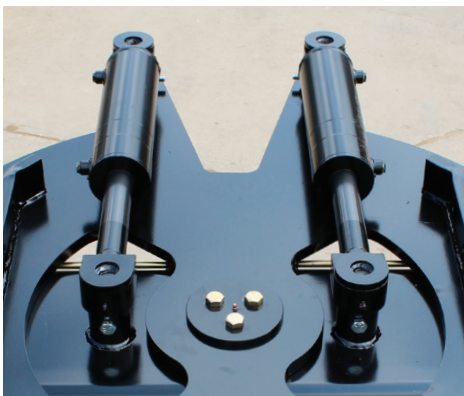
Reversing Cylinders: (2) provides a 45° working angle
