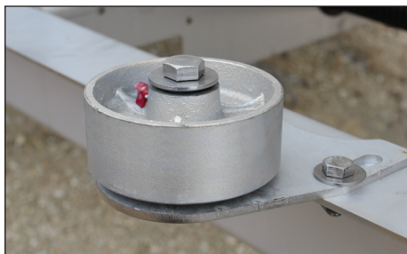
Standard front rollers guide while loading.
